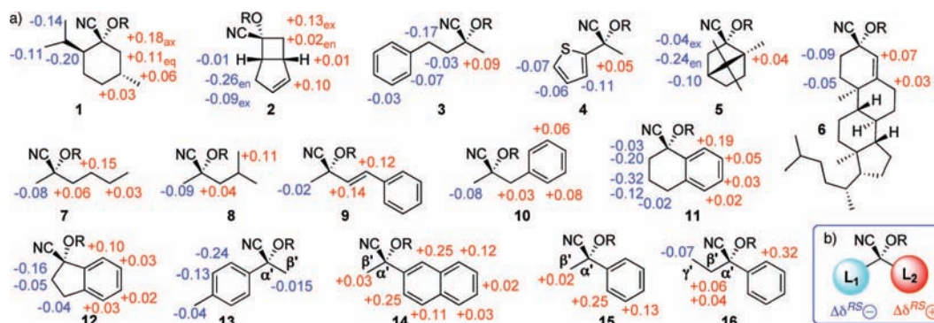
Figure 1. (a) \Delta\delta^{RS} values and signs for the MPA ester derivatives of ketone cyanohydrins 1–16 ( \text{CDCl}_3 ). (b) Spatial distribution of signs.
