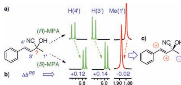
Figure 4. Steps to follow to assign the absolute configuration of ketone cyanohydrins using 9 as example.
