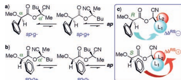
Figure 2. (a and b) Conformational equilibria for the ( R )- and ( S )-MPA esters of 7 ; (c) NMR significant conformers.
