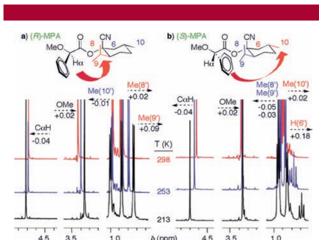
Figure 3. Temperature evolution of the 1 H NMR spectra of ( R )- and ( S )-MPA derivatives of 1 (a and b) and \Delta\delta^{T1/T2} values (ppm).
